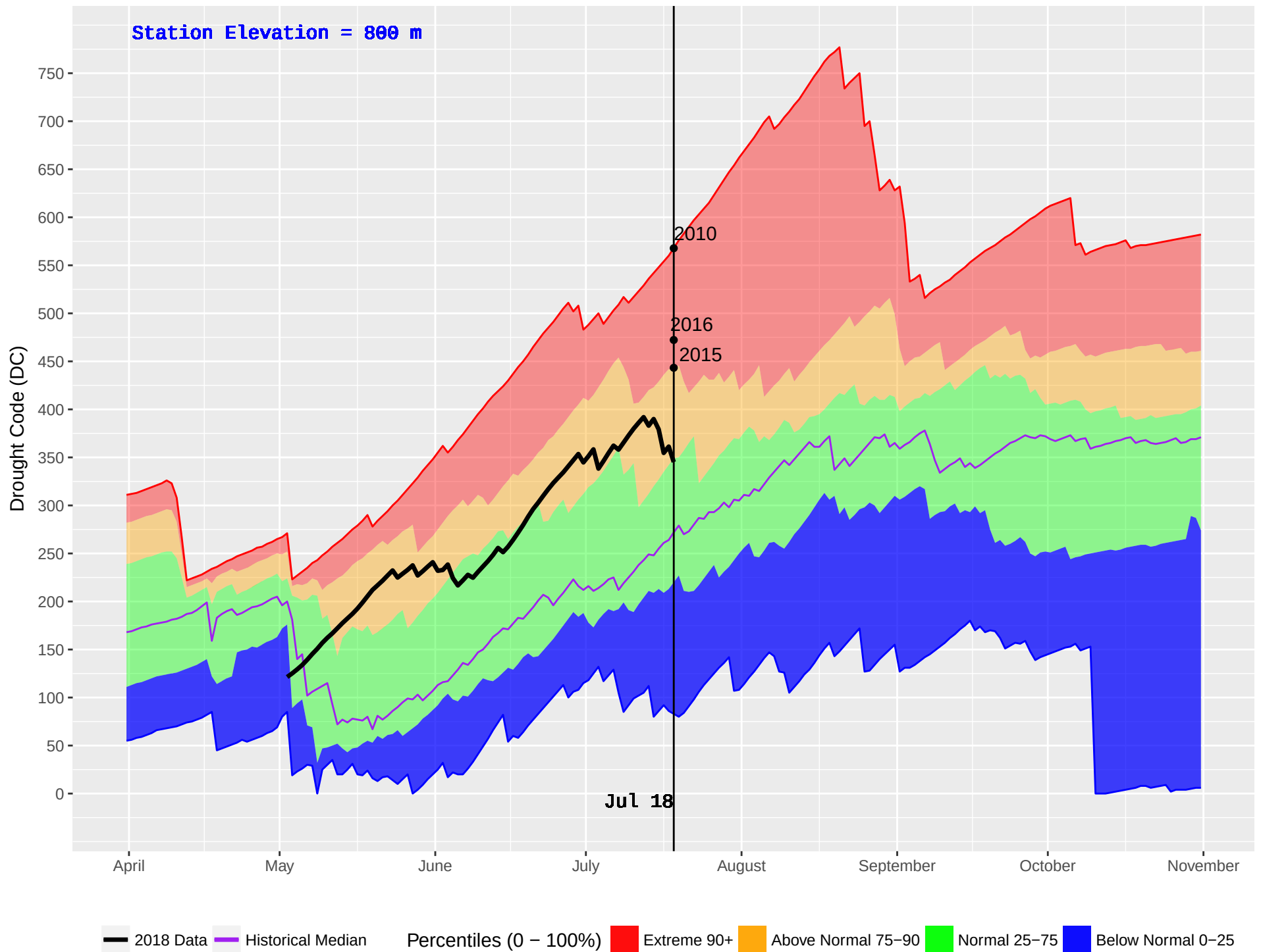
DEASE LAKE FS (108) : Historical (1978–2016) and Current (2018) Daily Drought Code (DC)
