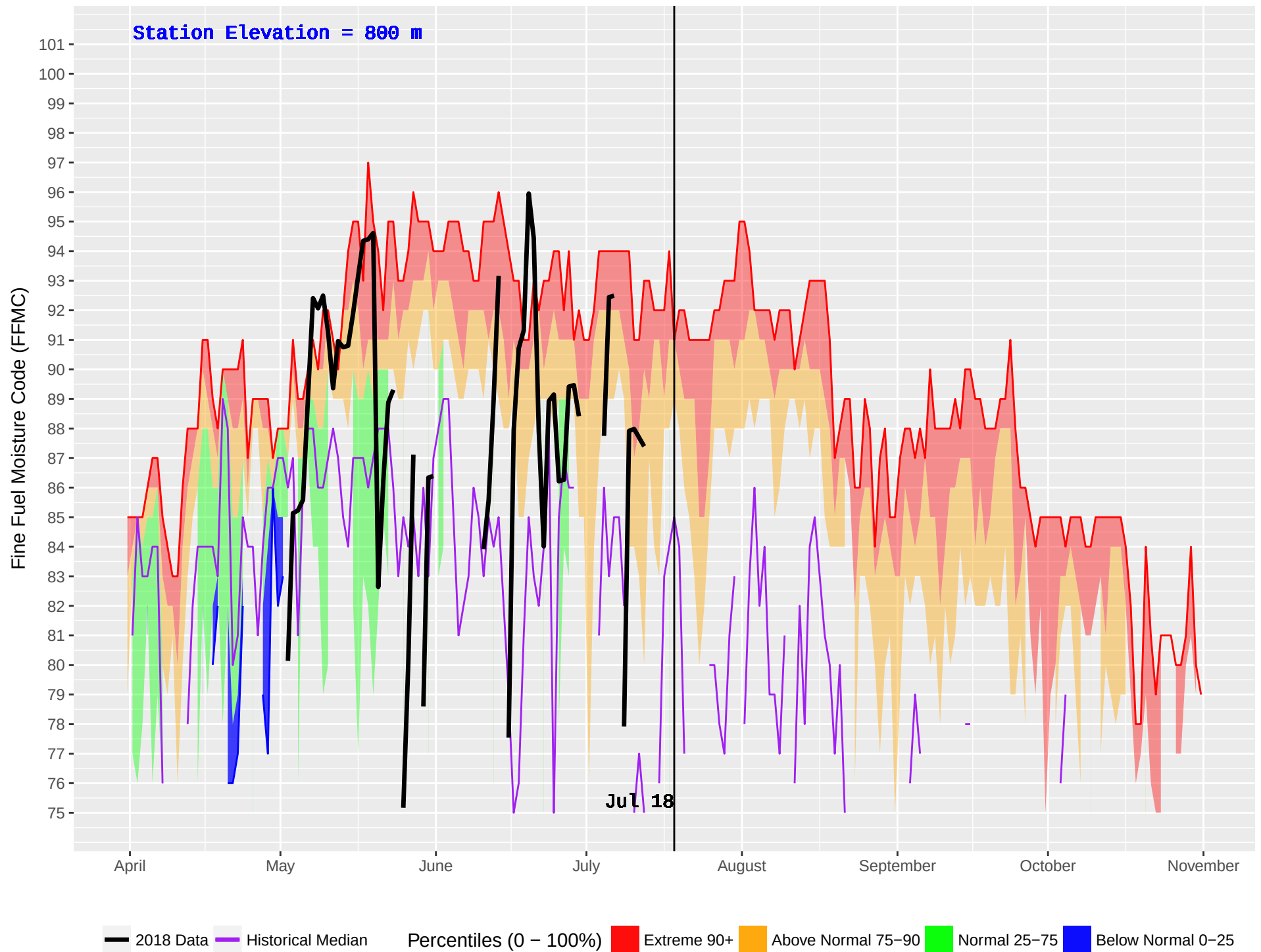
DEASE LAKE FS (108) : Historical (1978–2016) and Current (2018) Daily Fine Fuel Moisture Code (FFMC)
